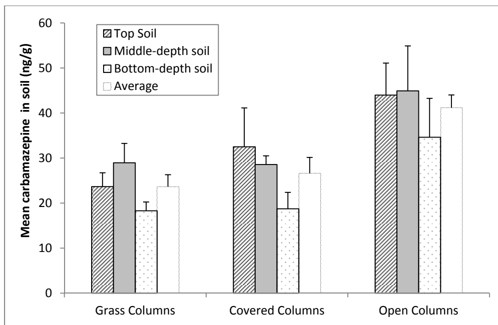
Figure 7: Comparison of carbamazepine concentration (mean \pm standard deviation) at different soil depths and different column types.
